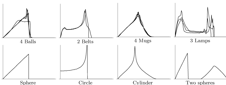
Fig. 14. D_2 shape distributions indicate the global shape of an object.
